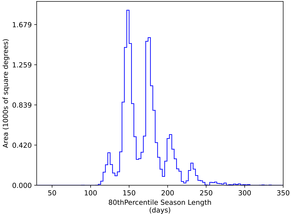
weather_cloudso4v3.4_10yrs WFD y band: 80thPercentile Season Length
