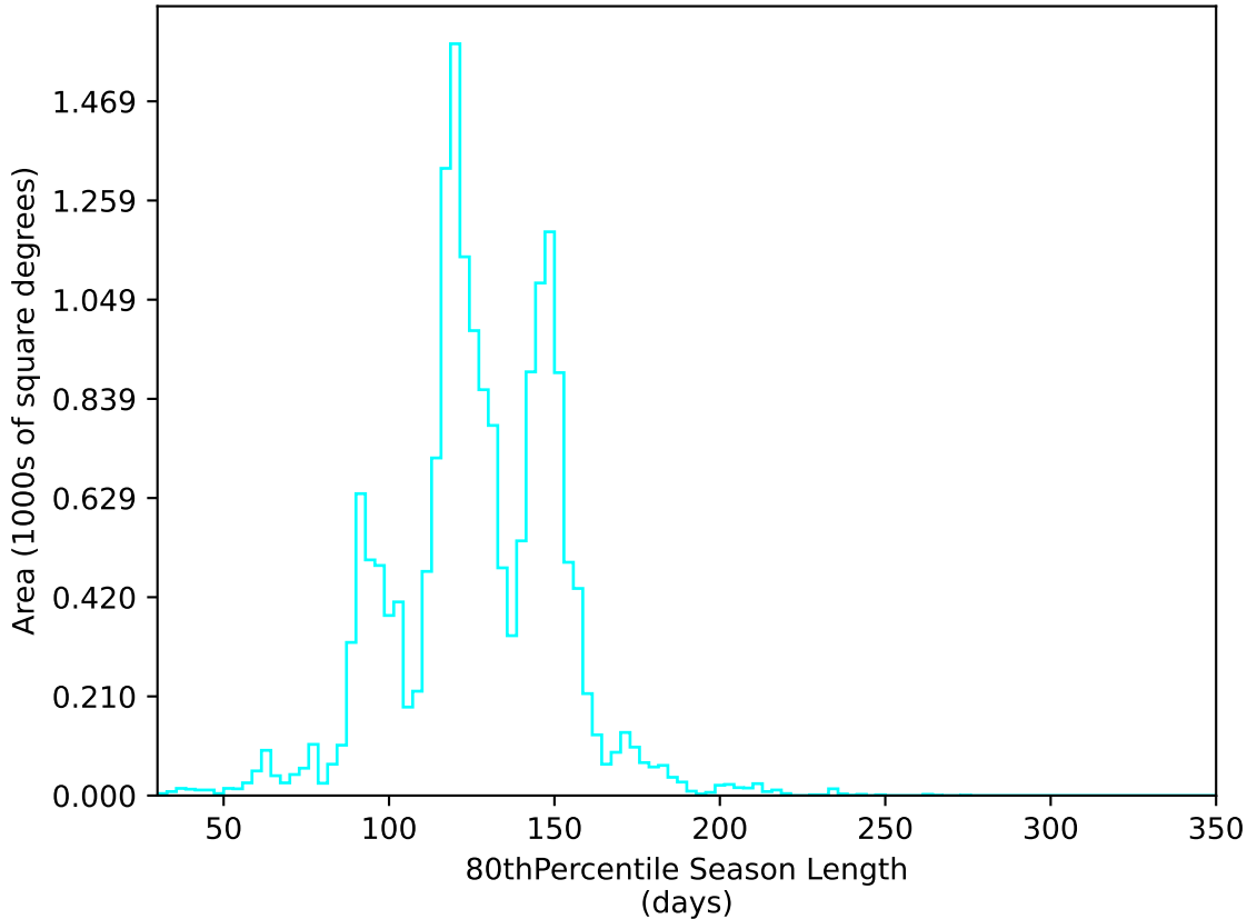
weather_cloudso4v3.4_10yrs WFD u band: 80thPercentile Season Length
