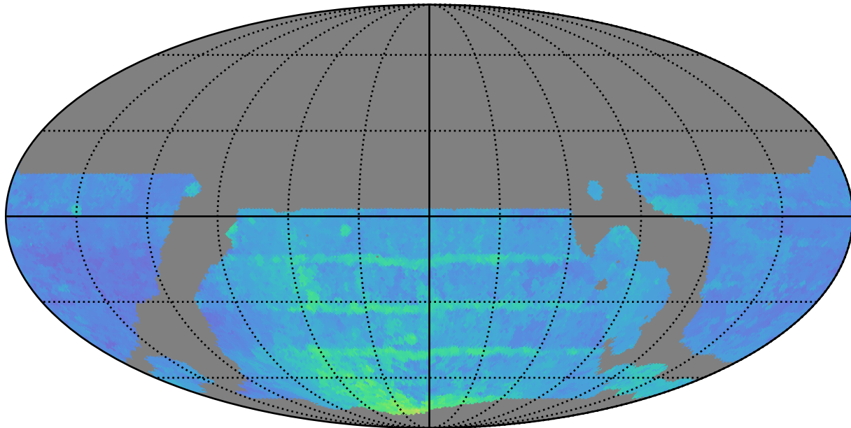
weather_cloudso4v3.4_10yrs WFD r band: 80thPercentile Season Length
