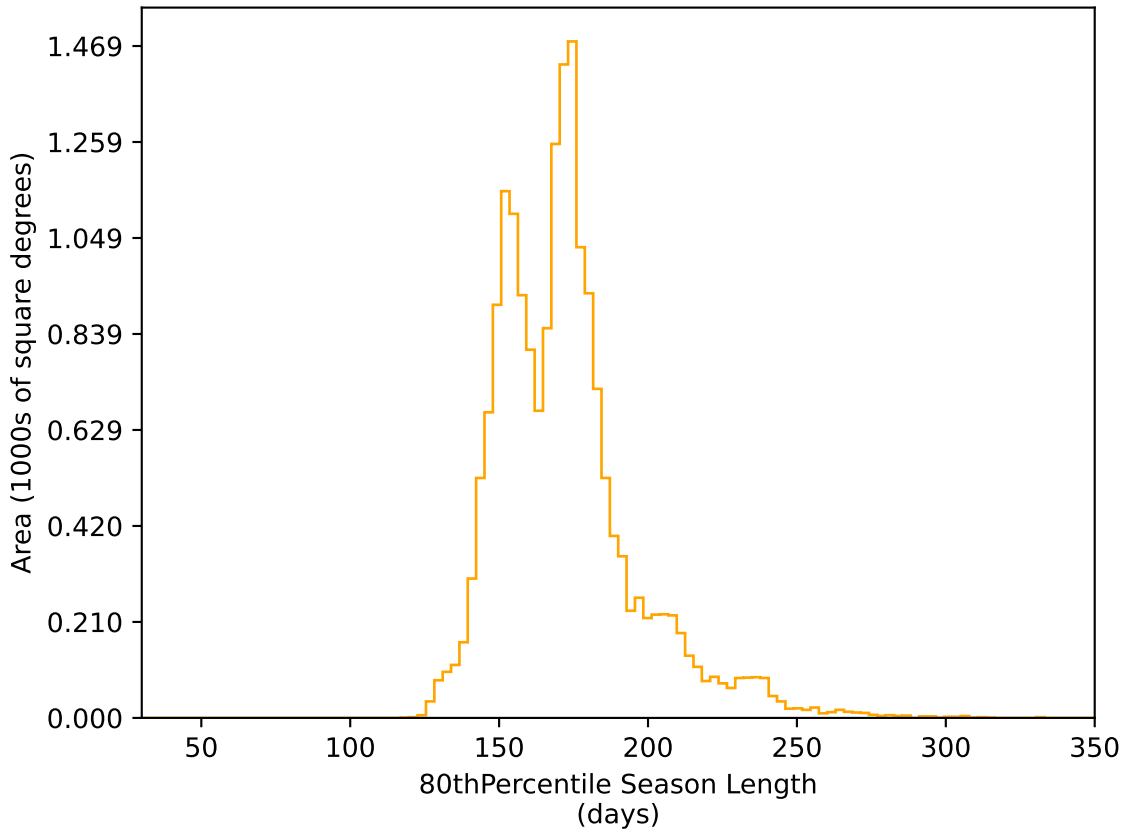
weather_cloudso4v3.4_10yrs WFD r band: 80thPercentile Season Length
