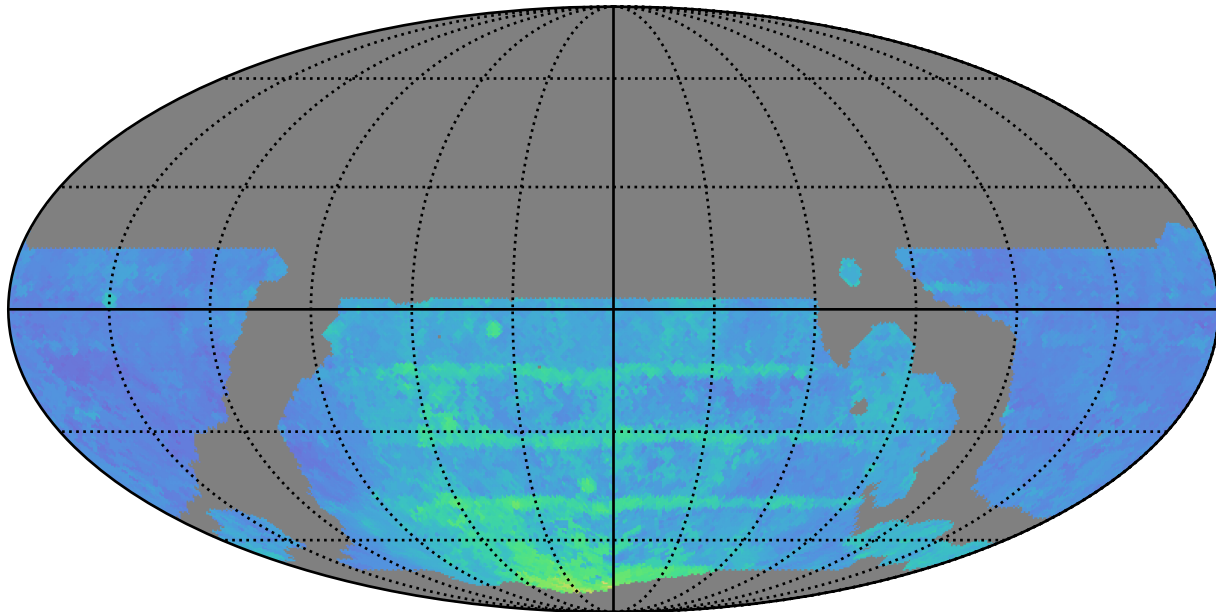
weather_cloudso4v3.4_10yrs WFD i band: 80thPercentile Season Length
