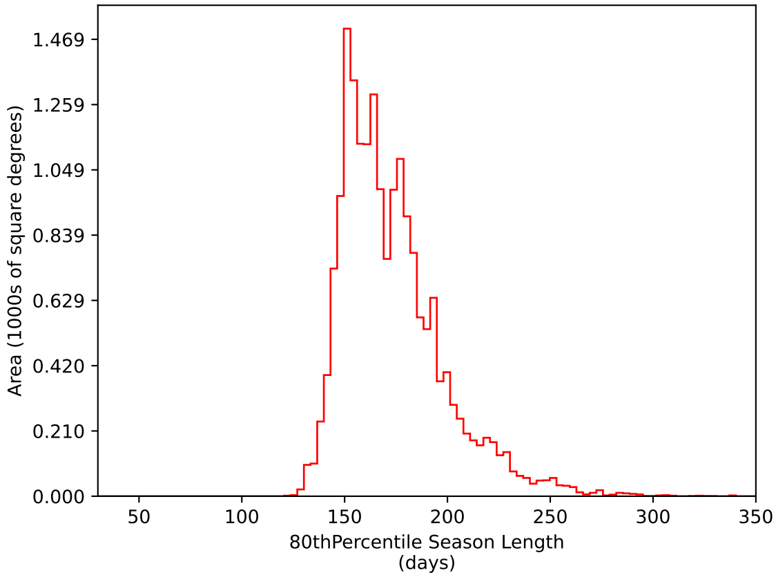
weather_cloudso4v3.4_10yrs WFD i band: 80thPercentile Season Length
