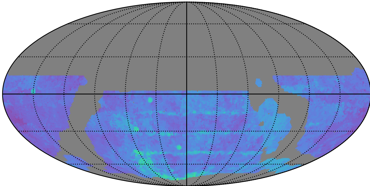
weather_cloudso4v3.4_10yrs WFD g band: 80thPercentile Season Length
