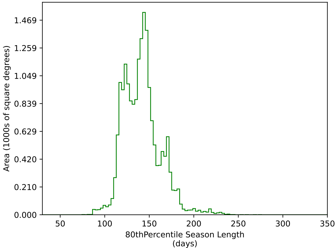
weather_cloudso4v3.4_10yrs WFD g band: 80thPercentile Season Length
