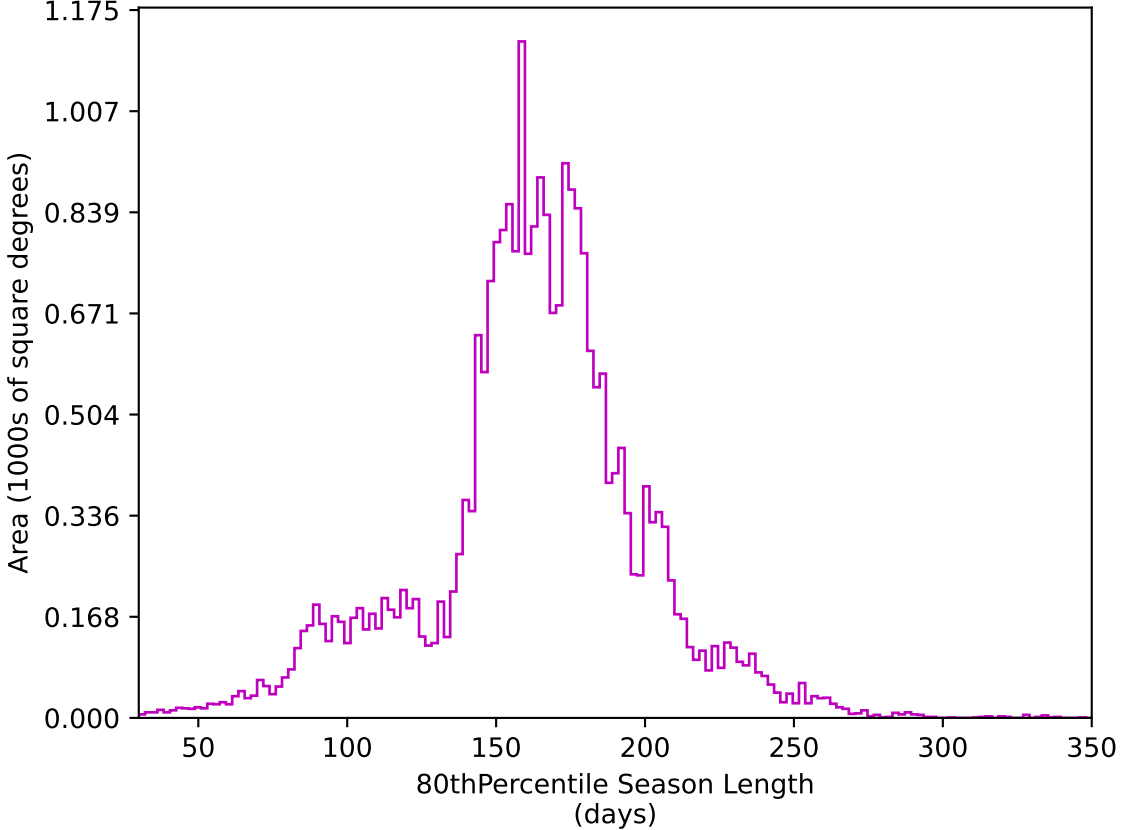
weather_cloudso4v3.4_10yrs All sky z band: 80thPercentile Season Length
