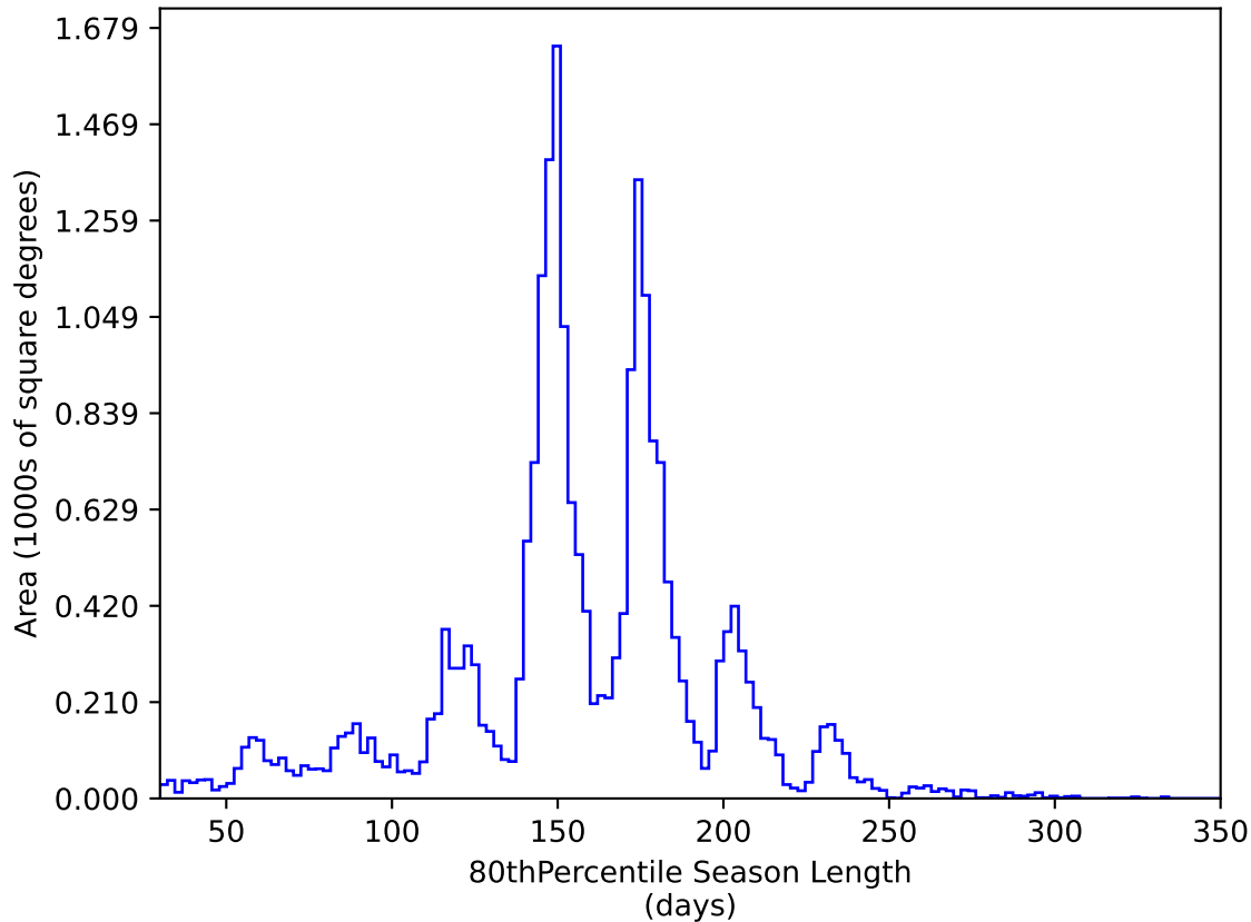
weather_cloudso4v3.4_10yrs All sky y band: 80thPercentile Season Length
