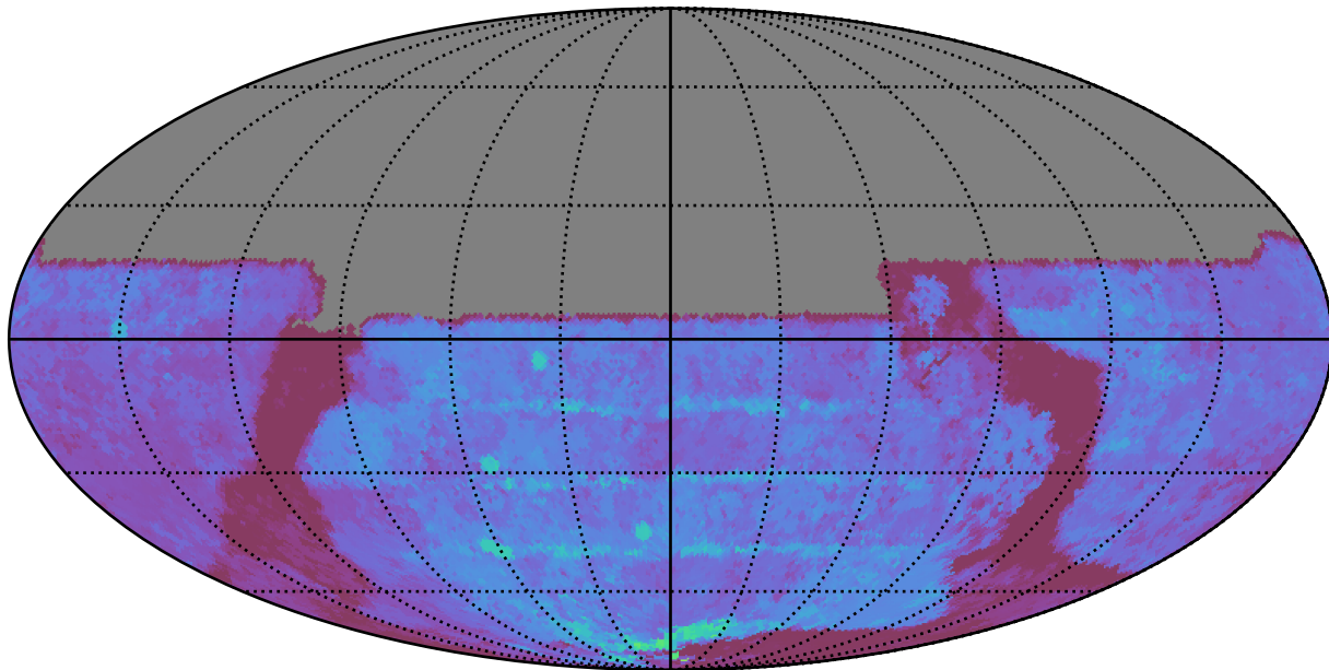
weather_cloudso4v3.4_10yrs All sky u band: 80thPercentile Season Length
