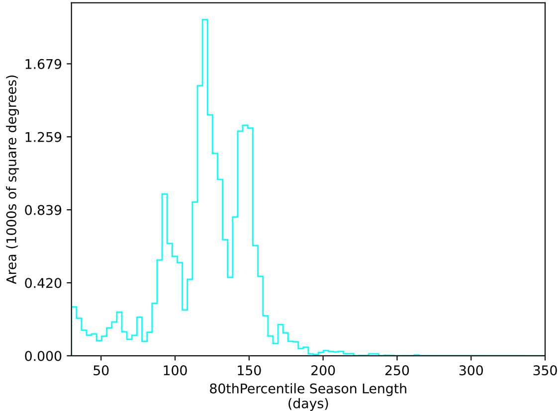
weather_cloudso4v3.4_10yrs All sky u band: 80thPercentile Season Length
