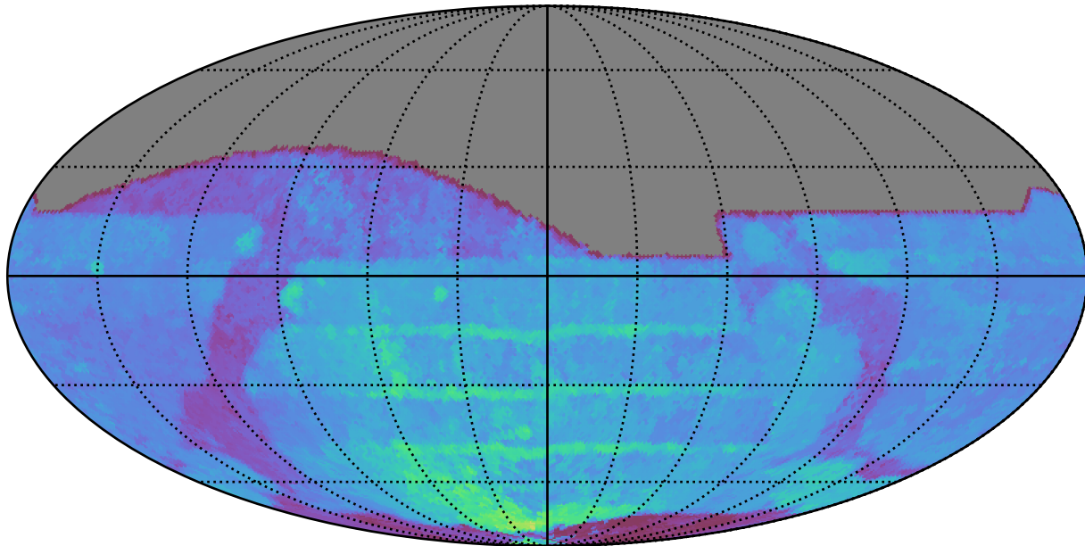
weather_cloudso4v3.4_10yrs All sky r band: 80thPercentile Season Length
