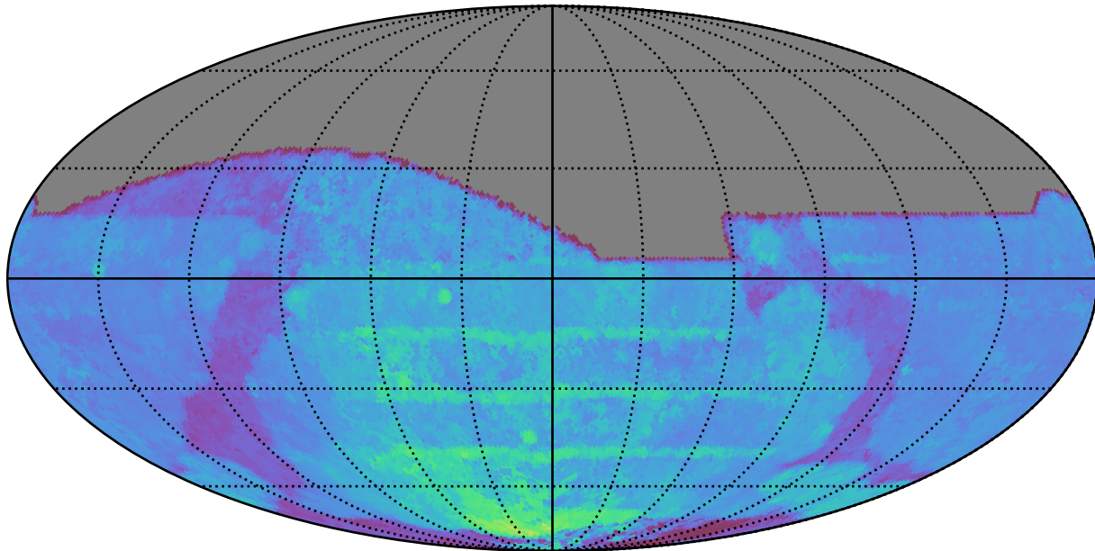
weather_cloudso4v3.4_10yrs All sky i band: 80thPercentile Season Length
