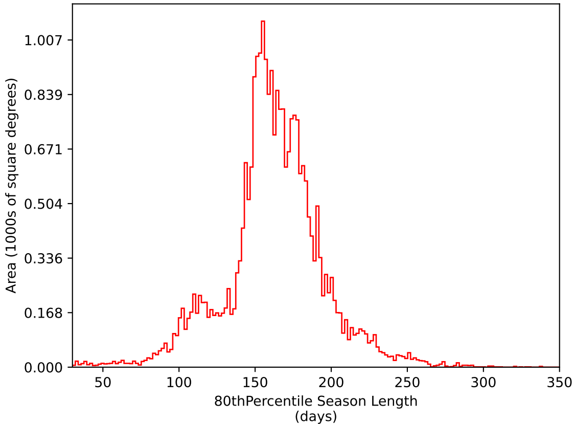
weather_cloudso4v3.4_10yrs All sky i band: 80thPercentile Season Length
