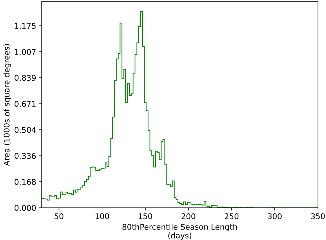
weather_cloudso4v3.4_10yrs All sky g band: 80thPercentile Season Length
