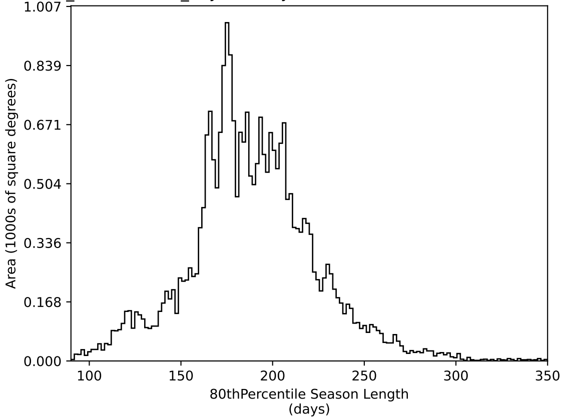
weather_cloudso4v3.4_10yrs All sky all bands: 80thPercentile Season Length
