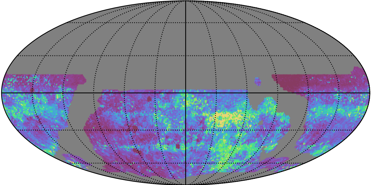
weather_cloudso4v3.4_10yrs WFD zy bands: 75th Percentile Intranight Timespan
