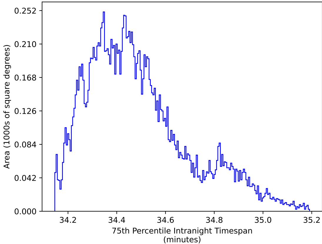
weather_cloudso4v3.4_10yrs WFD zy bands: 75th Percentile Intranight Timespan
