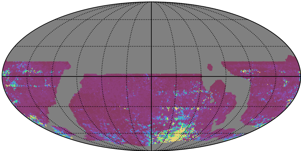
weather_cloudso4v3.4_10yrs WFD z band: 75th Percentile Intranight Timespan
