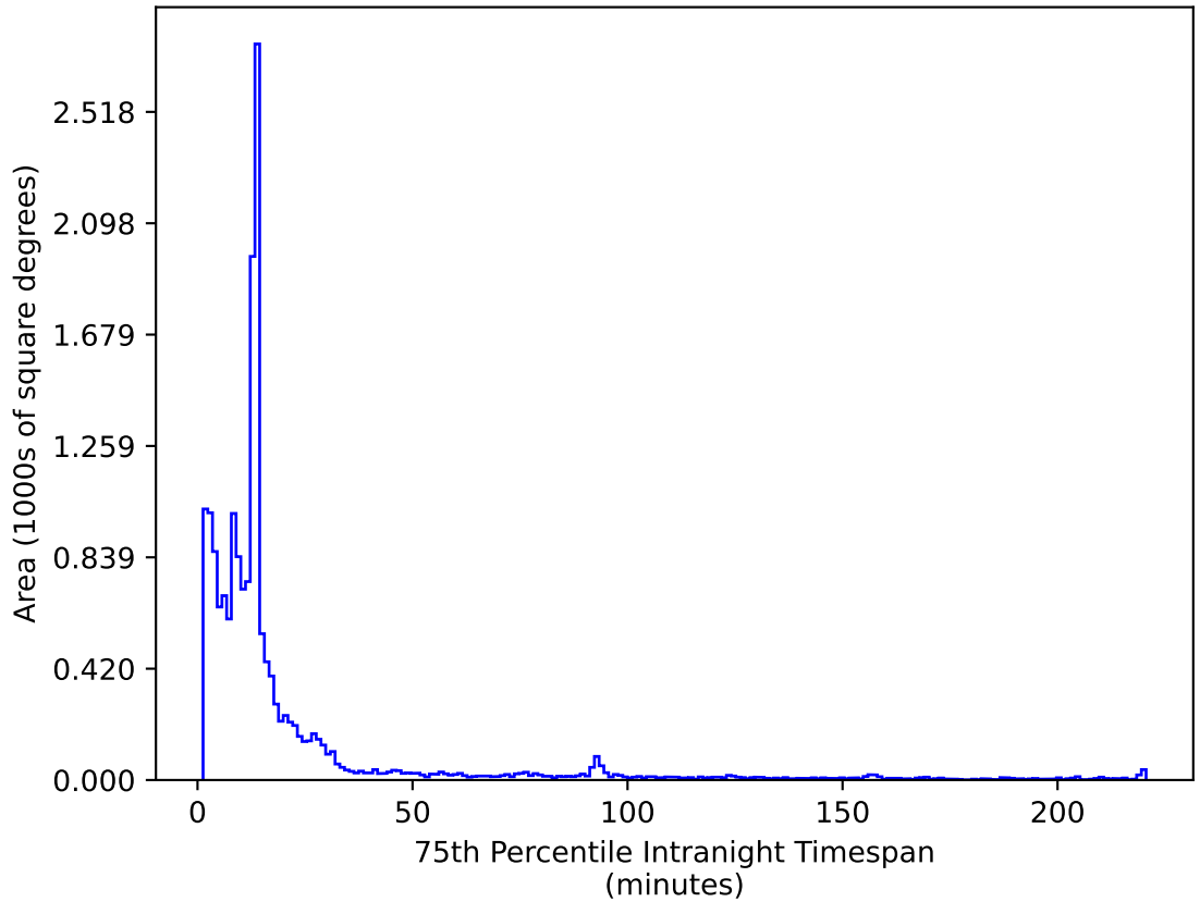
weather_cloudso4v3.4_10yrs WFD z band: 75th Percentile Intranight Timespan
