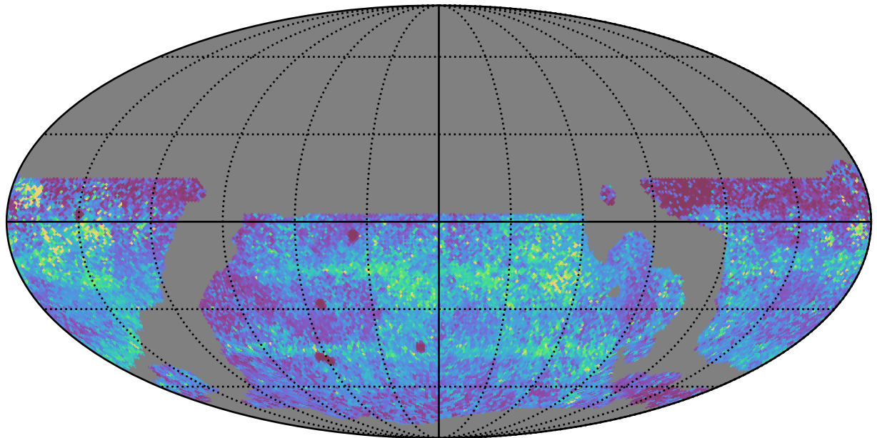
weather_cloudso4v3.4_10yrs WFD y band: 75th Percentile Intranight Timespan
