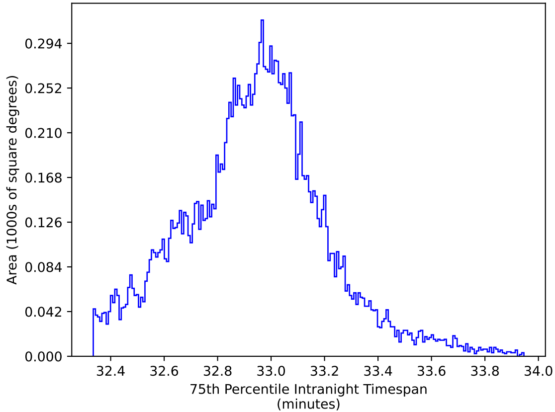
weather_cloudso4v3.4_10yrs WFD y band: 75th Percentile Intranight Timespan
