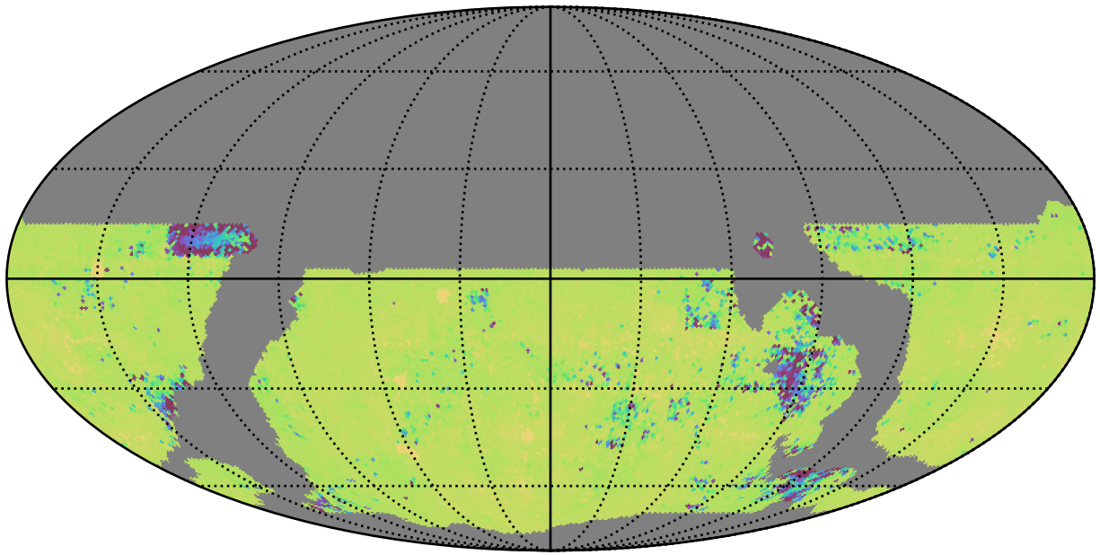
weather_cloudso4v3.4_10yrs WFD ug bands: 75th Percentile Intranight Timespan
