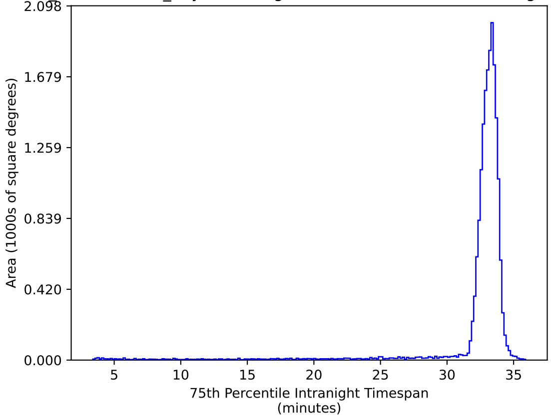
weather_cloudso4v3.4_10yrs WFD ug bands: 75th Percentile Intranight Timespan
