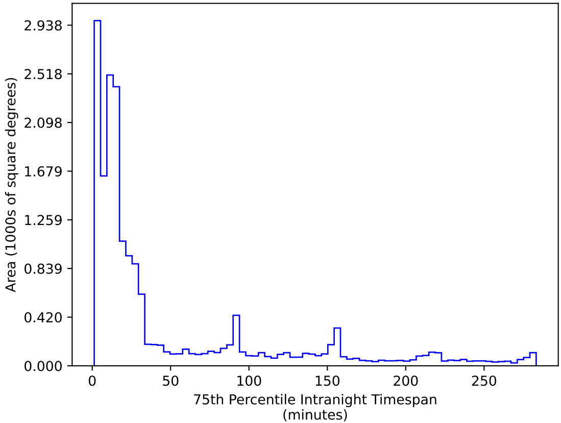
weather_cloudso4v3.4_10yrs WFD r band: 75th Percentile Intranight Timespan
