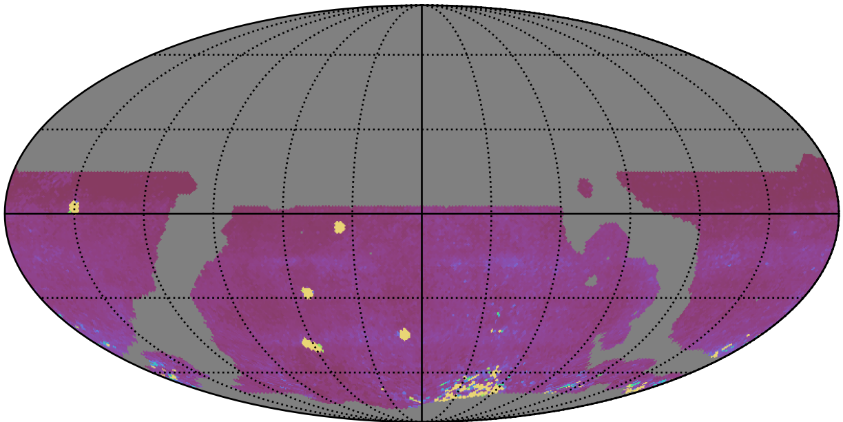
weather_cloudso4v3.4_10yrs WFD iz bands: 75th Percentile Intranight Timespan
