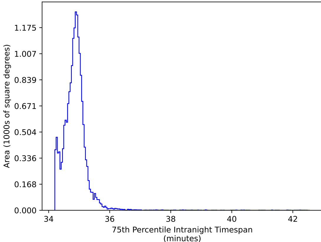
weather_cloudso4v3.4_10yrs WFD iz bands: 75th Percentile Intranight Timespan
