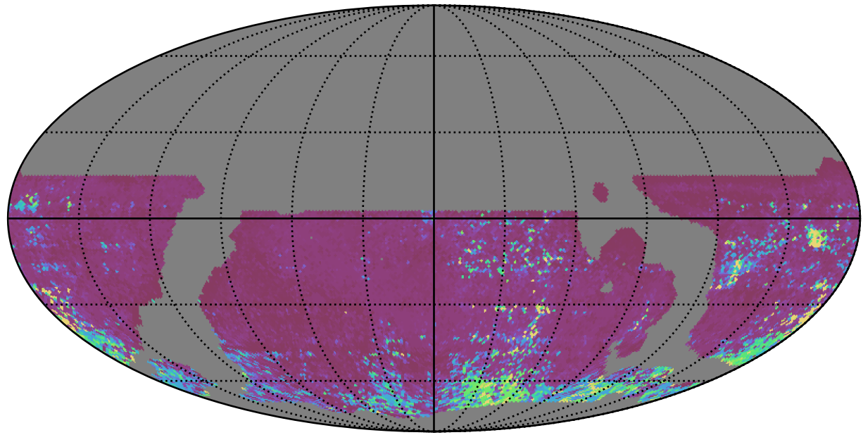
weather_cloudso4v3.4_10yrs WFD i band: 75th Percentile Intranight Timespan
