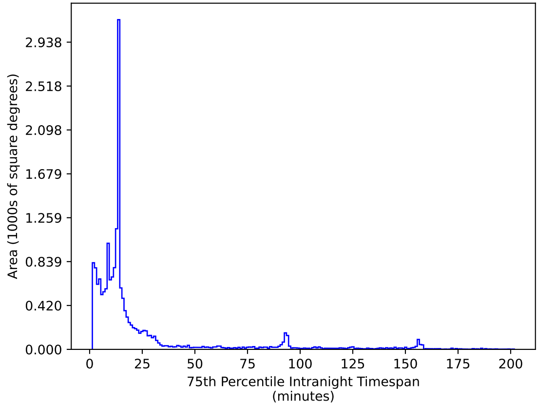
weather_cloudso4v3.4_10yrs WFD i band: 75th Percentile Intranight Timespan
