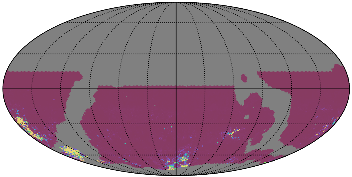
weather_cloudso4v3.4_10yrs WFD gr bands: 75th Percentile Intranight Timespan
