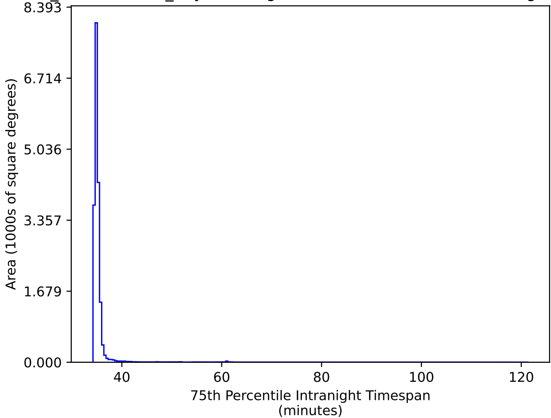
weather_cloudso4v3.4_10yrs WFD gr bands: 75th Percentile Intranight Timespan
