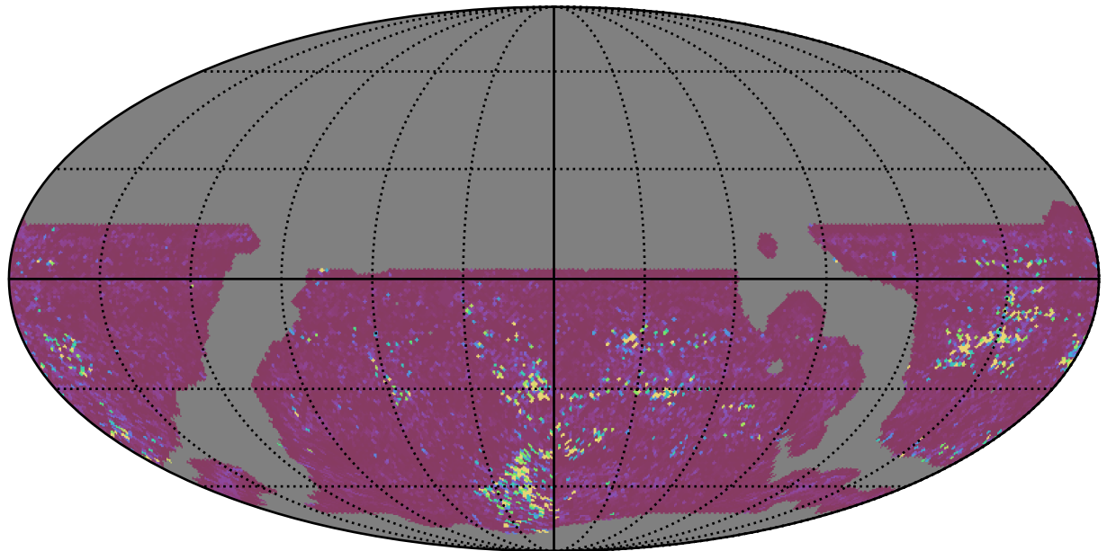
weather_cloudso4v3.4_10yrs WFD g band: 75th Percentile Intranight Timespan
