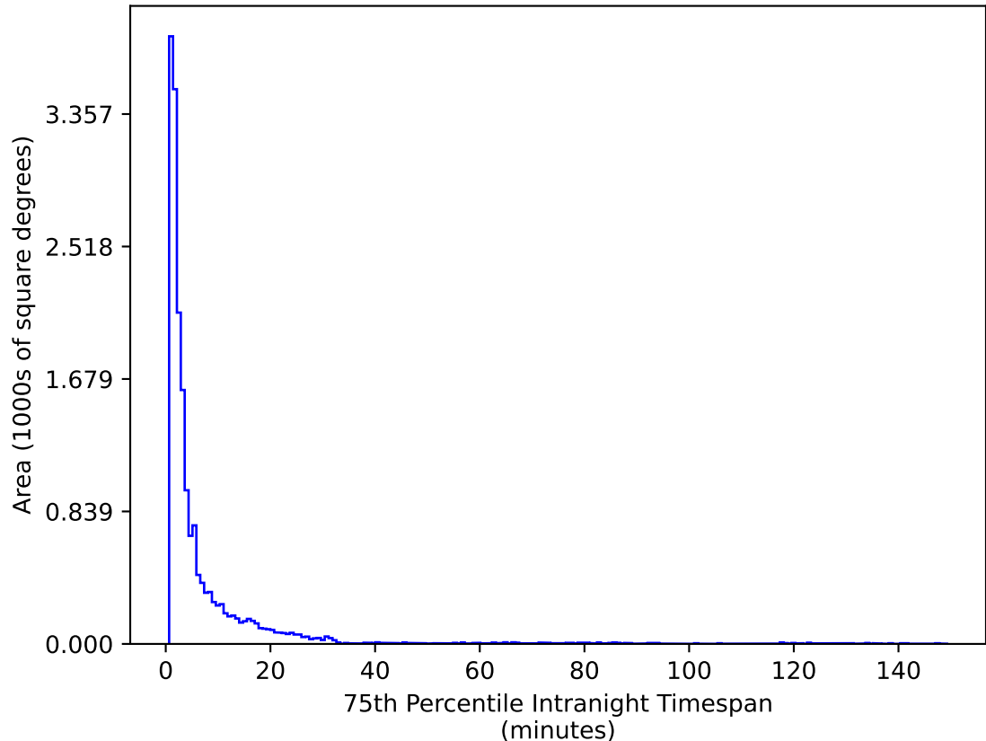
weather_cloudso4v3.4_10yrs WFD g band: 75th Percentile Intranight Timespan
