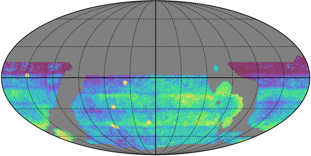
weather_cloudso4v3.4_10yrs WFD all bands: 75th Percentile Intranight Timespan
