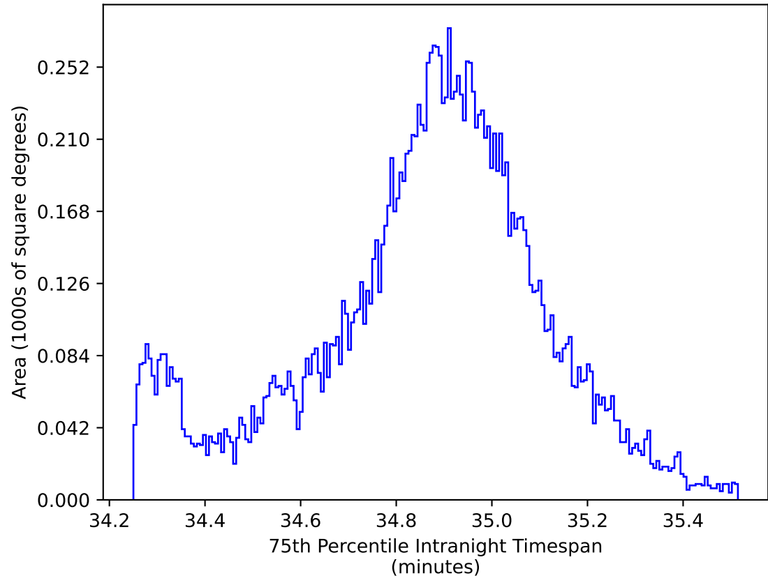
weather_cloudso4v3.4_10yrs WFD all bands: 75th Percentile Intranight Timespan
