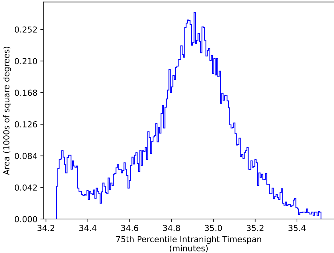
weather_cloudso4v3.4_10yrs WFD: 75th Percentile Intranight Timespan
