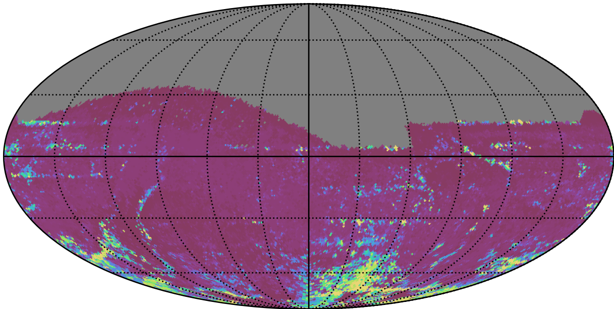
weather_cloudso4v3.4_10yrs All sky z band: 75th Percentile Intranight Timespan
