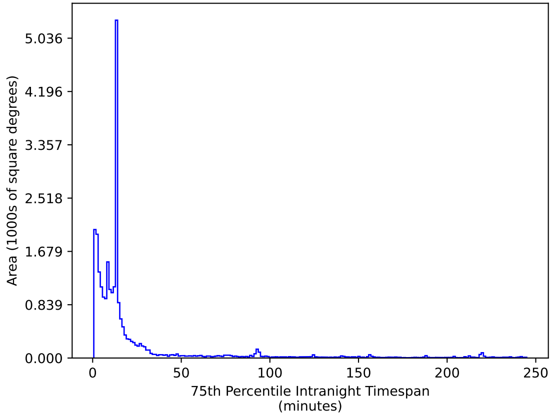
weather_cloudso4v3.4_10yrs All sky z band: 75th Percentile Intranight Timespan
