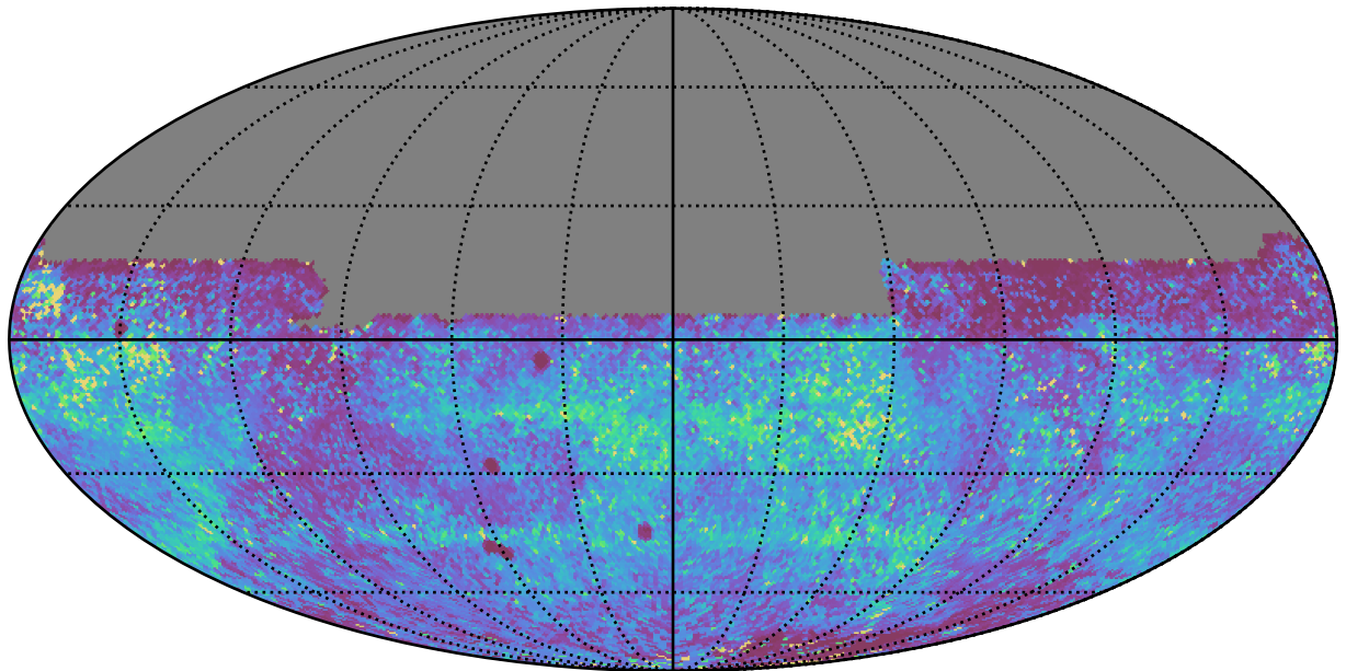
weather_cloudso4v3.4_10yrs All sky y band: 75th Percentile Intranight Timespan
