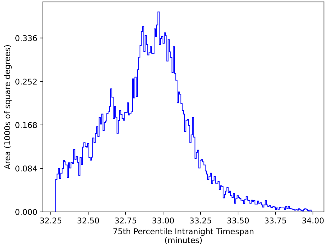
weather_cloudso4v3.4_10yrs All sky y band: 75th Percentile Intranight Timespan
