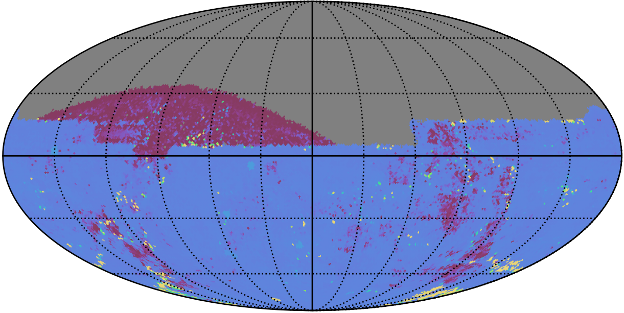
weather_cloudso4v3.4_10yrs All sky ug bands: 75th Percentile Intranight Timespan
