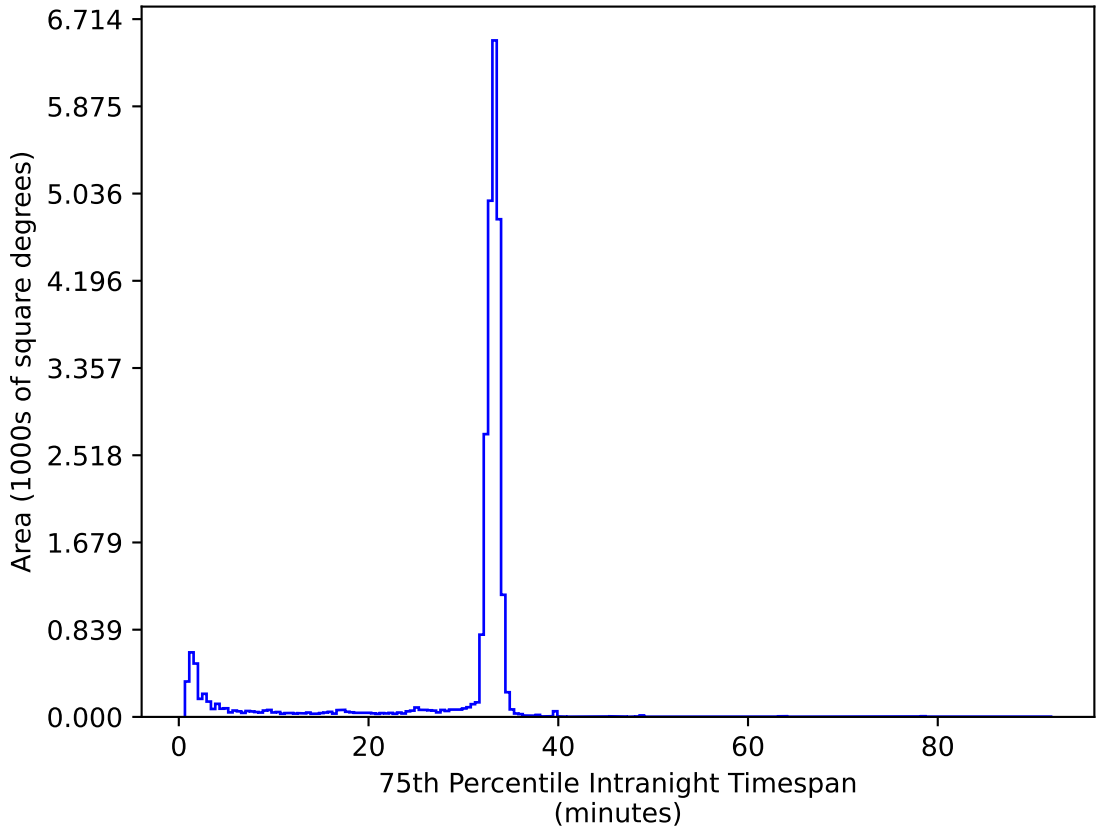
weather_cloudso4v3.4_10yrs All sky ug bands: 75th Percentile Intranight Timespan
