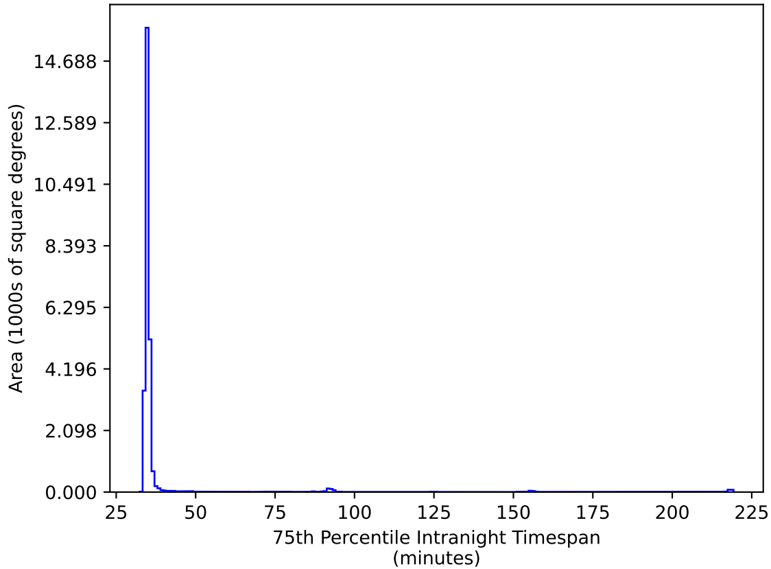
weather_cloudso4v3.4_10yrs All sky ri bands: 75th Percentile Intranight Timespan
