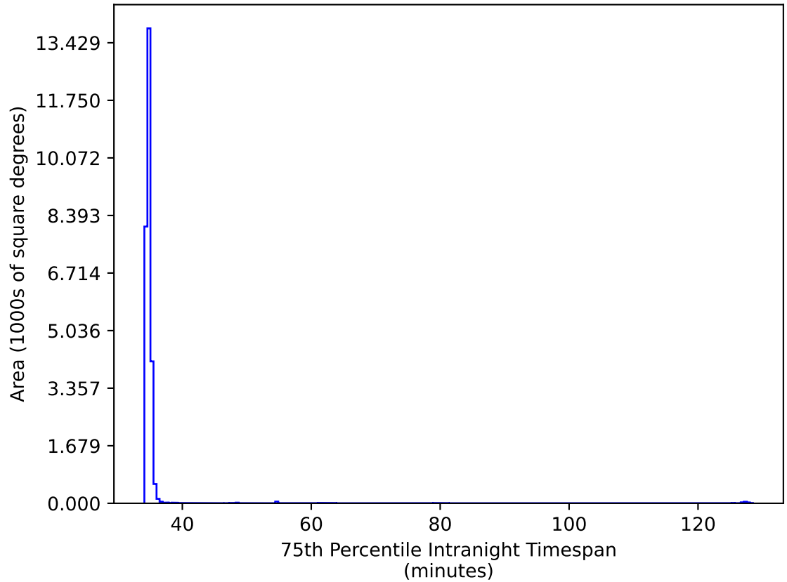
weather_cloudso4v3.4_10yrs All sky iz bands: 75th Percentile Intranight Timespan
