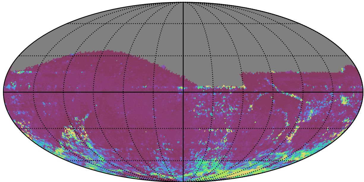
weather_cloudso4v3.4_10yrs All sky i band: 75th Percentile Intranight Timespan
