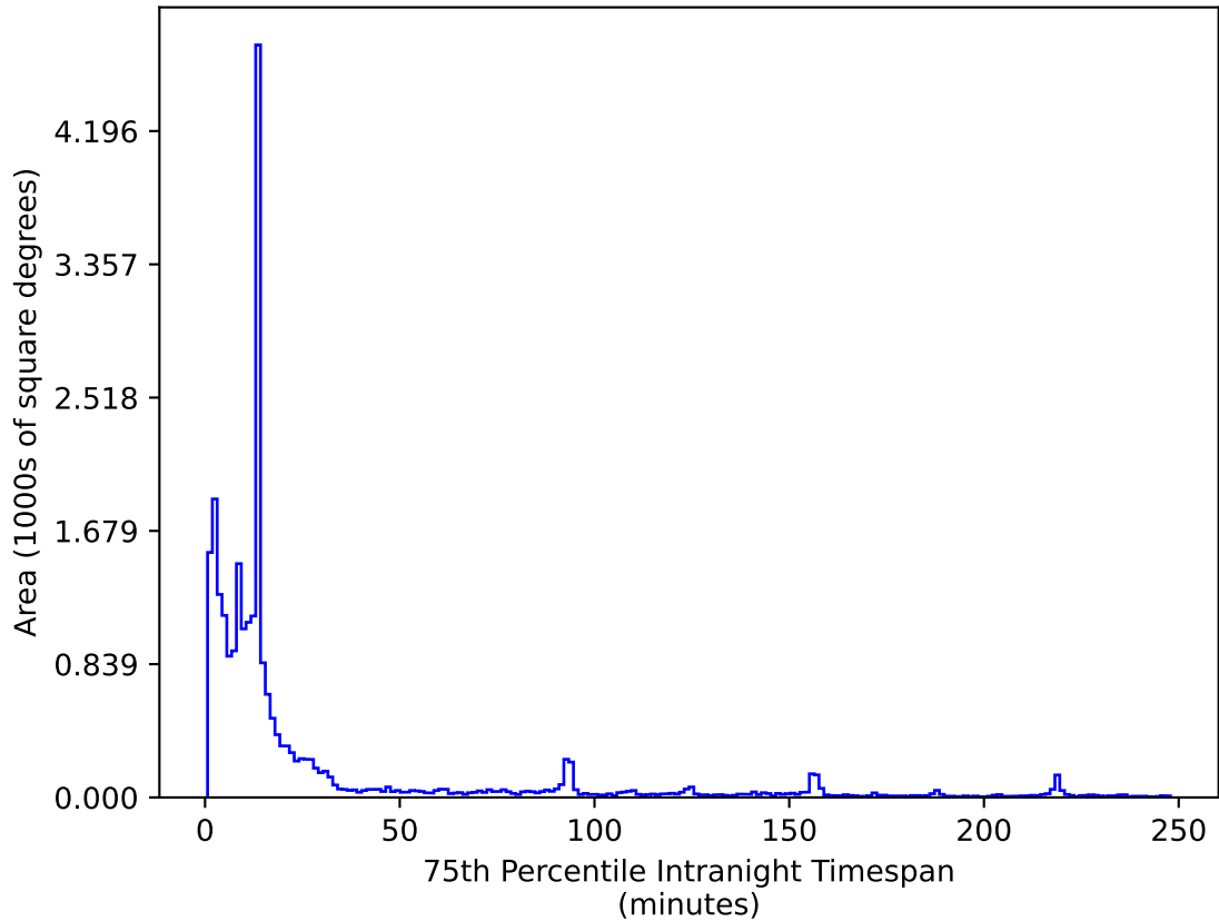
weather_cloudso4v3.4_10yrs All sky i band: 75th Percentile Intranight Timespan
