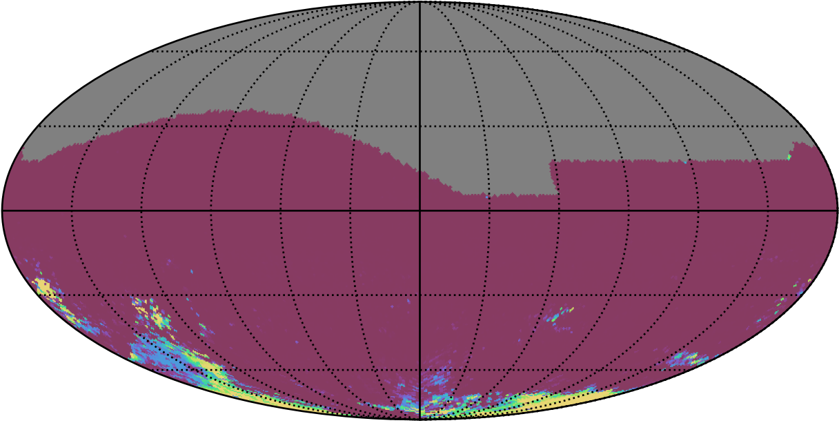
weather_cloudso4v3.4_10yrs All sky gr bands: 75th Percentile Intranight Timespan
