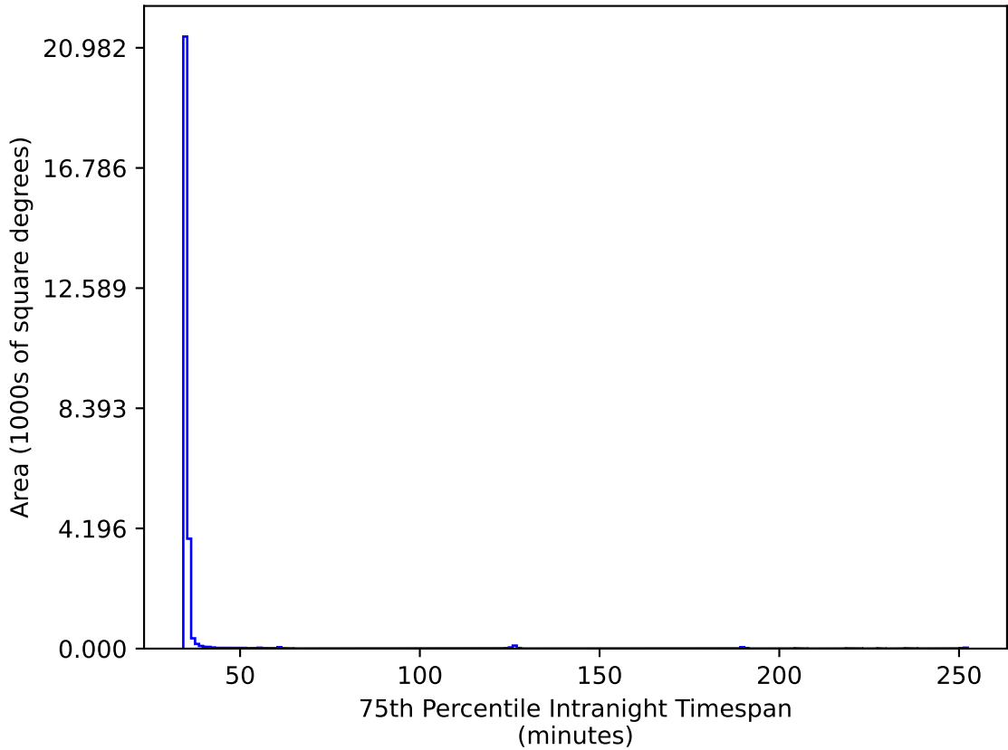
weather_cloudso4v3.4_10yrs All sky gr bands: 75th Percentile Intranight Timespan
