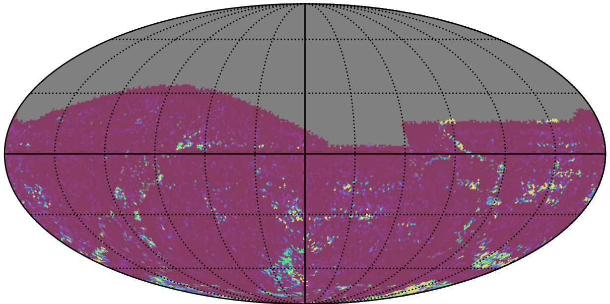
weather_cloudso4v3.4_10yrs All sky g band: 75th Percentile Intranight Timespan
